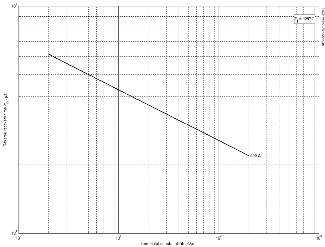
Fig 8 - Recovery time, t_{rr} (50% chord)
