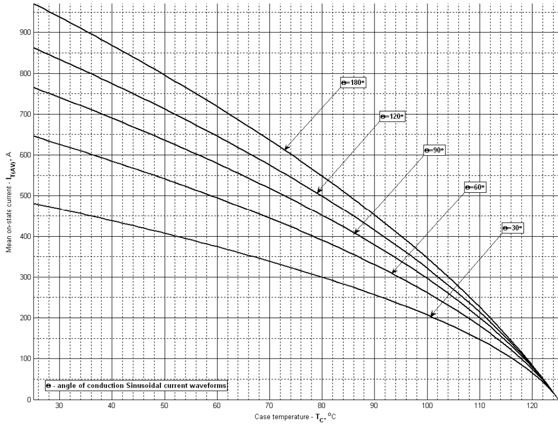
Fig 11 – Maximum case temperature (sinusoidal current waveforms)
