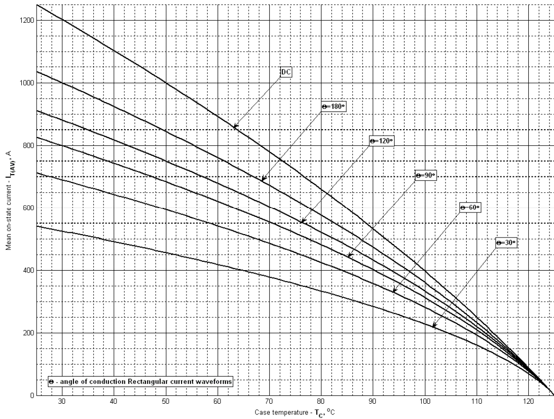
Fig 12 - Maximum case temperature (rectangular current waveforms)
