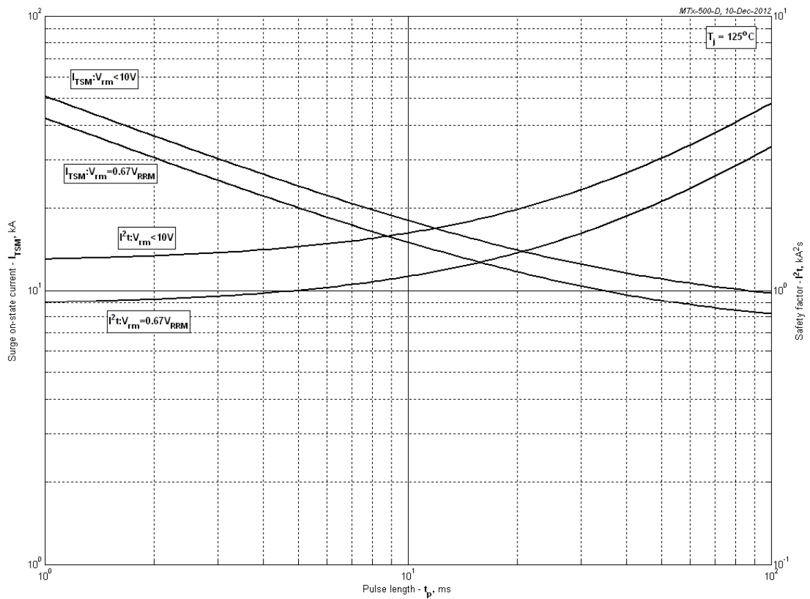
Fig 14 - Maximum surge ratings
