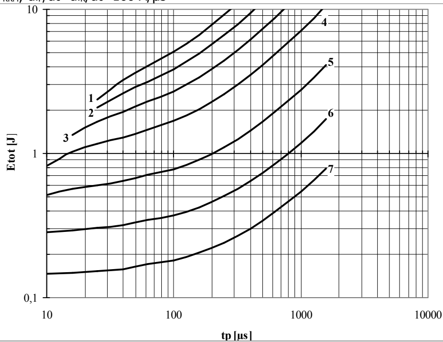
Fig. 27 Square wave loss energy per pulse
