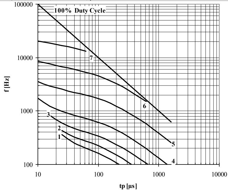
Fig. 17 Square wave frequency ratings
