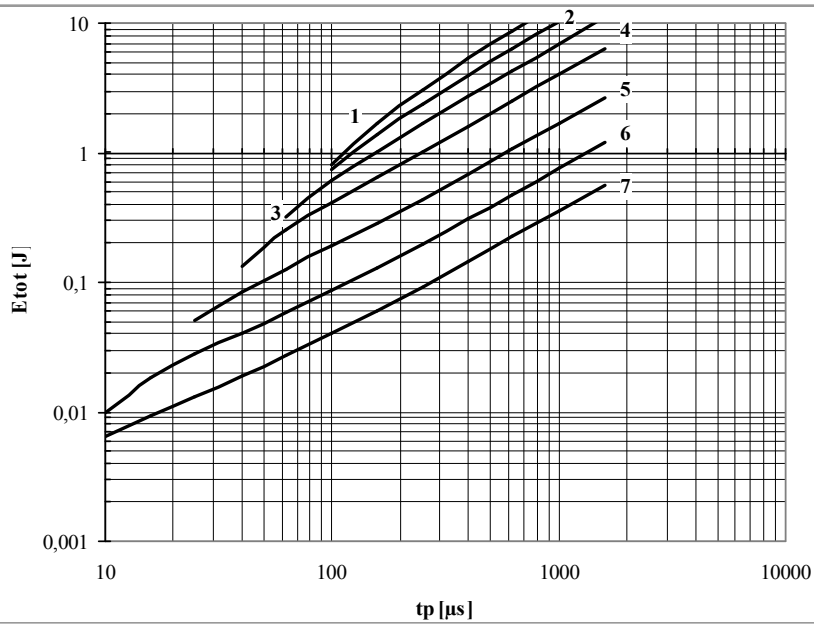
Fig. 24 Square wave loss energy per pulse
