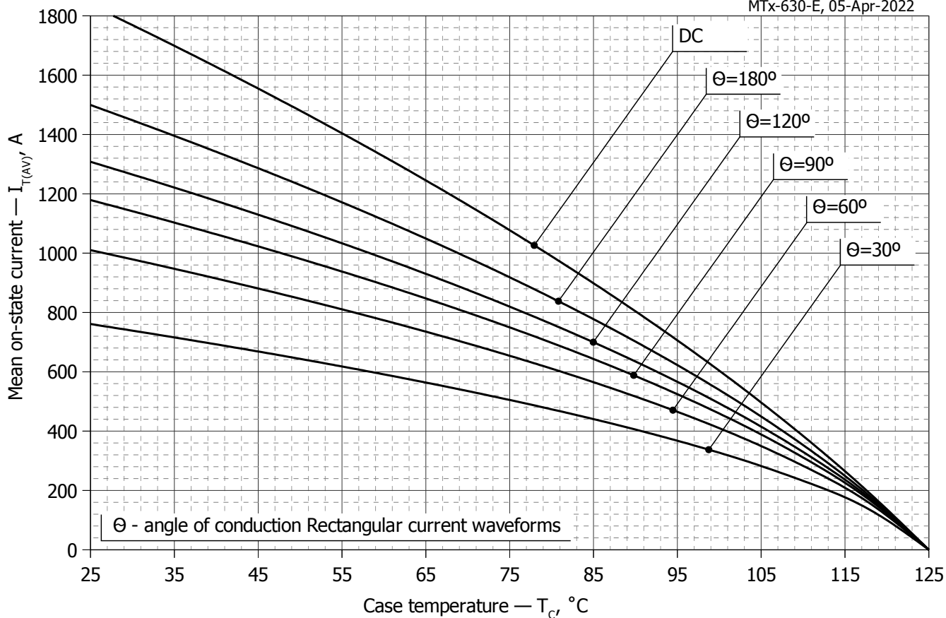
Fig. 12 - Mean on-state current I_{TAV} vs. case temperature T_c for rectangular current waveforms at different conduction angles and for DC (f=50Hz, DSC)
