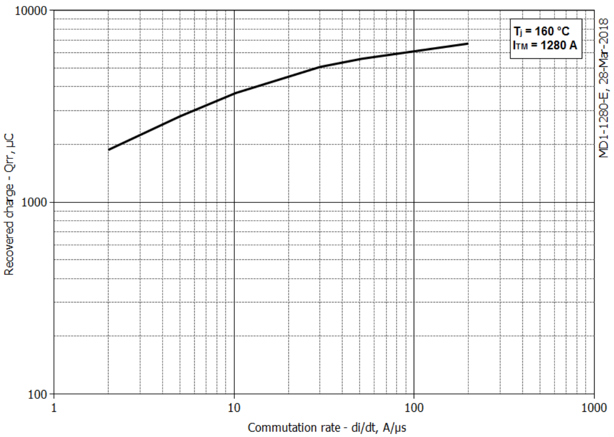
Fig 4 - Recovered charge, Q_{rr} (25% chord)
