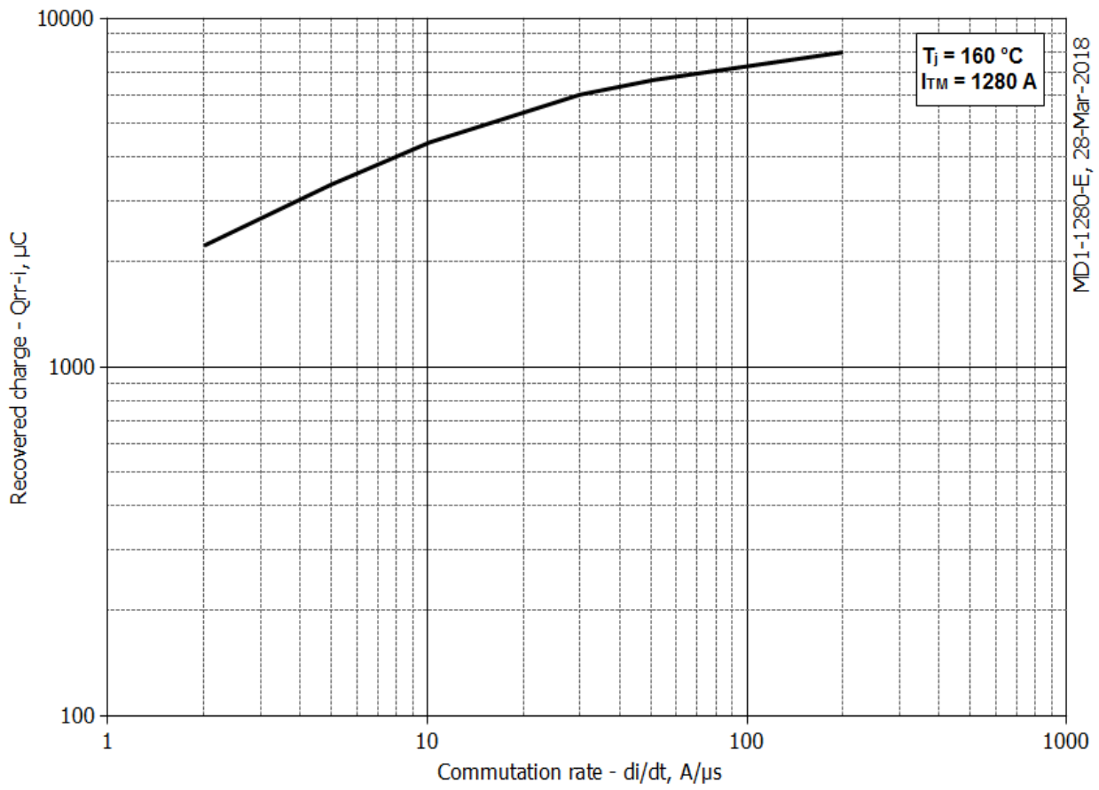
Fig 3 – Total recovered charge, Q_{rr-i} (integral)
