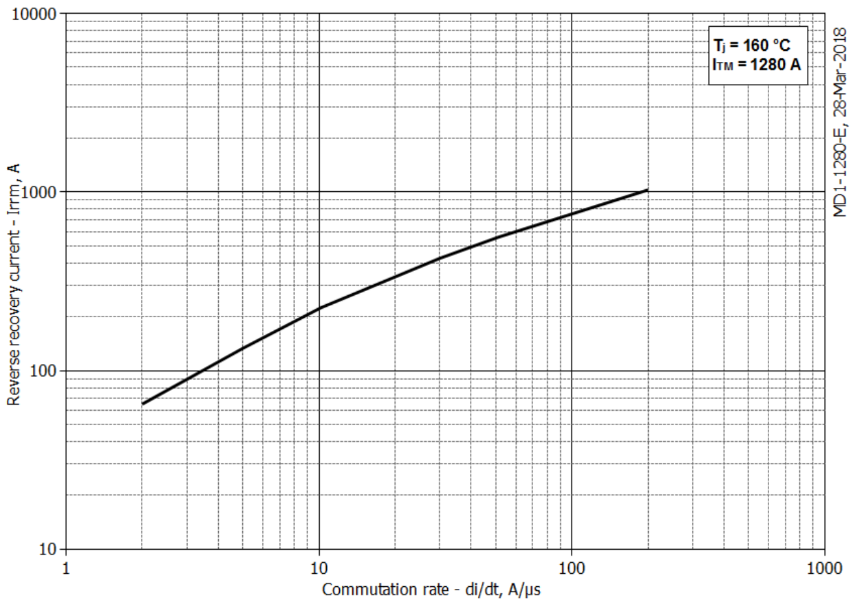
Fig 5 – Peak reverse recovery current, I_{rrm}
