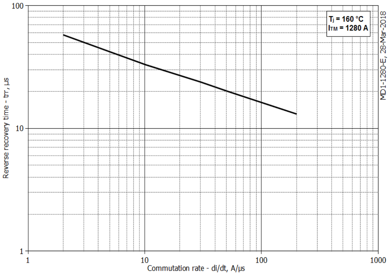
Fig 6 – Maximum recovery time, t_{rr} (25% chord)
